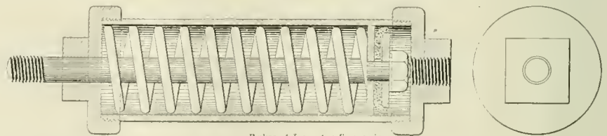
PNEUMATIC BELT SHIFTER.
